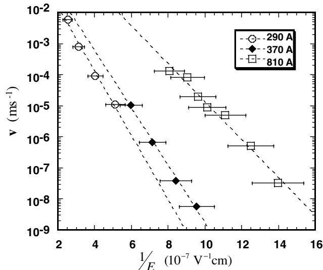
FIG. 3. Domain wall speed as a function of the inverse applied electric field for 290, 370, and 810 Å thick samples. The data fit well to v \sim \exp[-\frac{R}{k_B T} (\frac{E_0}{E})^\mu] with \mu = 1 , characteristic of a creep process.
